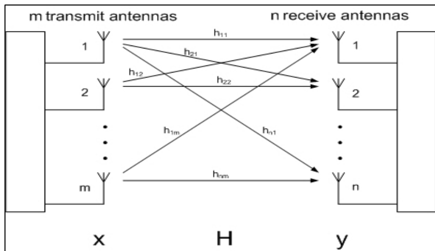
Figure 1 MIMO - Multiple Input Multiple Output (Poole, 2019)
