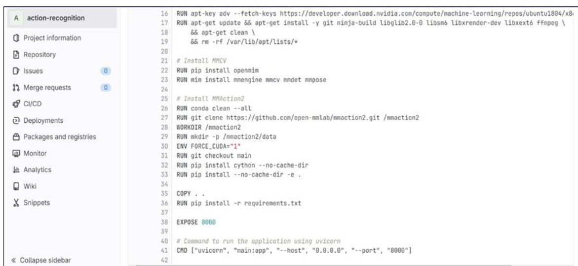
Figure 4 Containerization of model using docker
